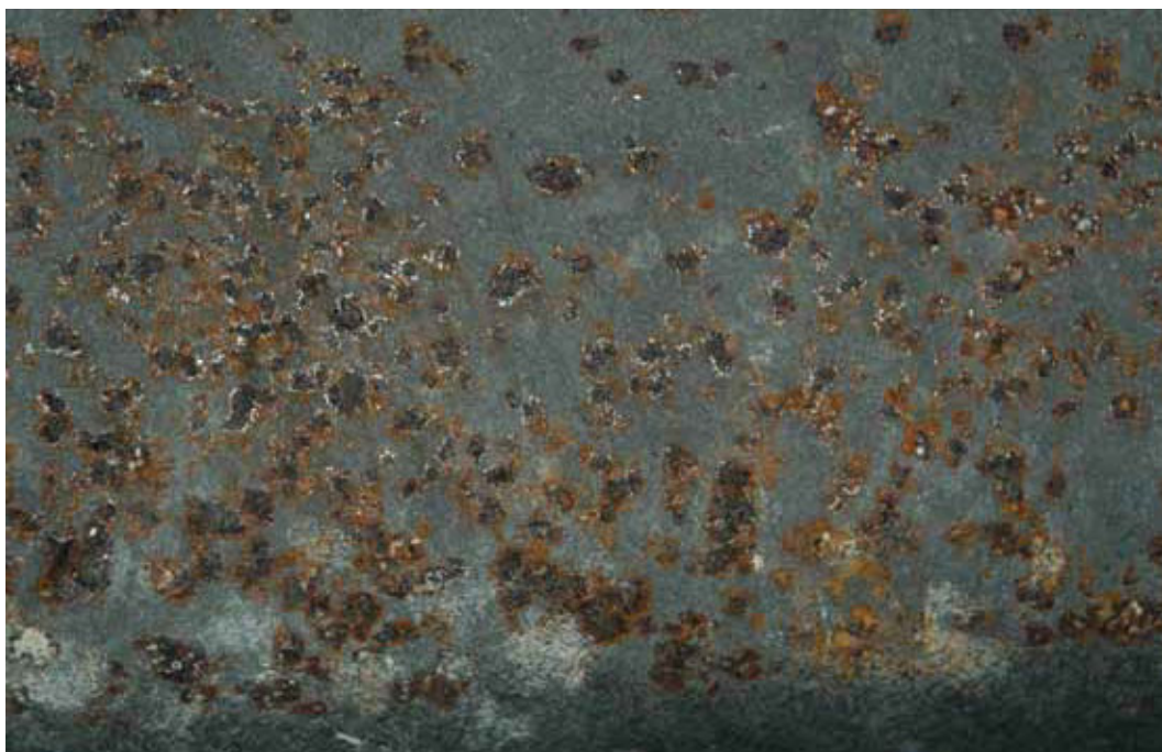
^ Typical pitting corrosion
