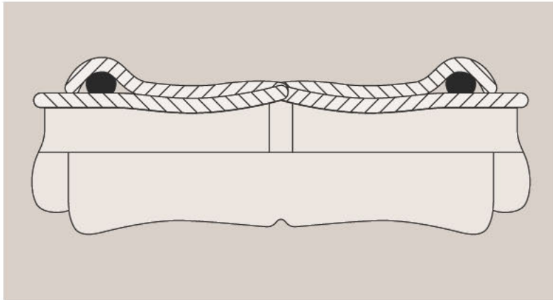
^ Typical push fit (press type) fitting
