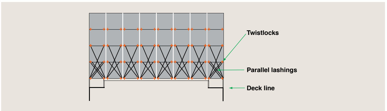
^ Containers secured by twistlocks and lashing rods. Lashing rods to bottom of third tier
