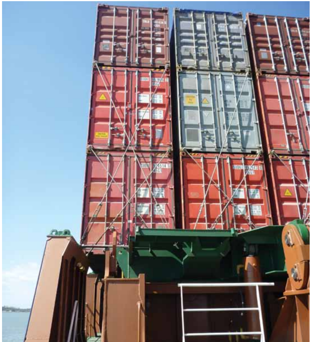
^ Outboard containers with lashings to the bottom of second and third tier boxes
