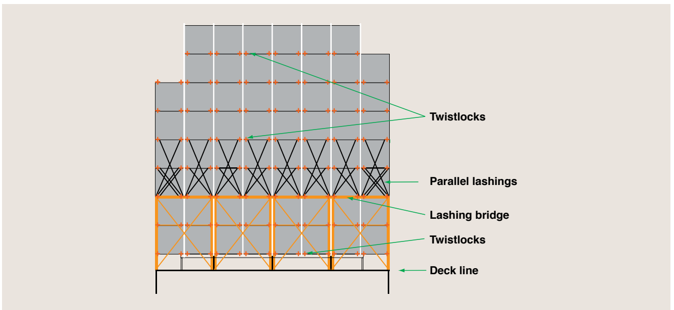
^ As above but lashings originate from a lashing bridge. Lashing rods to bottom of fifth tier
