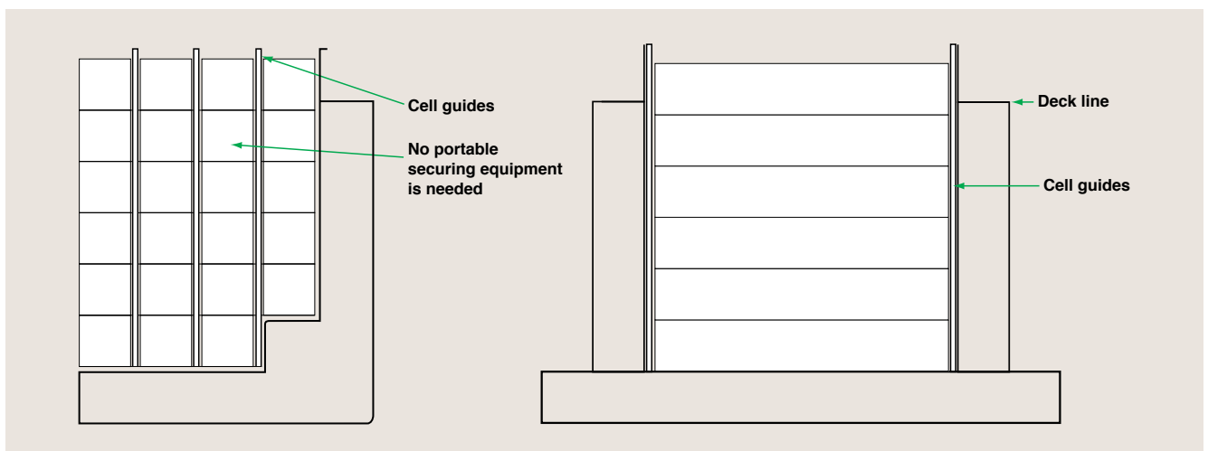
^ 40-foot containers in 40-foot cell guides
