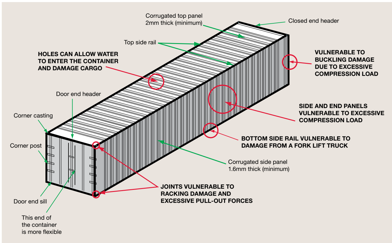
^ Container construction and faults
