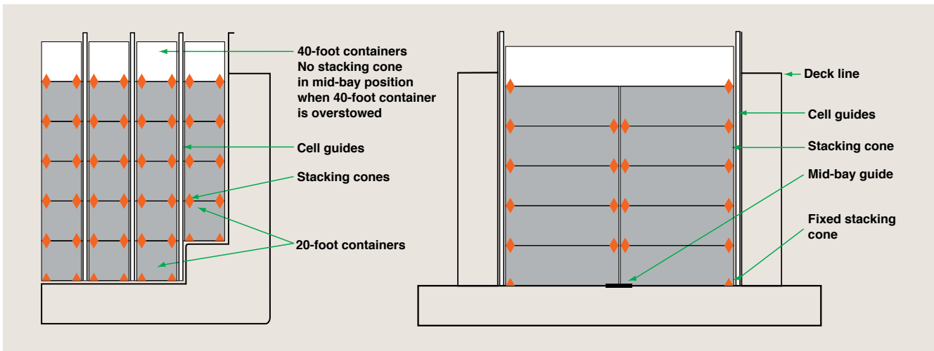
^ 20-foot containers in 40-foot cell guides with 40-foot containers stowed above
