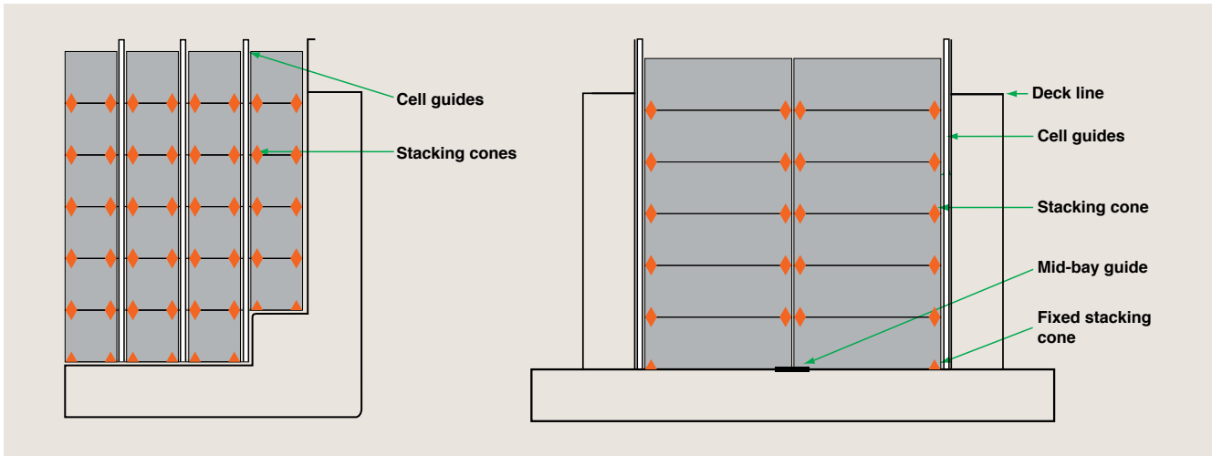
^ 20-foot containers in 40-foot cell guides
