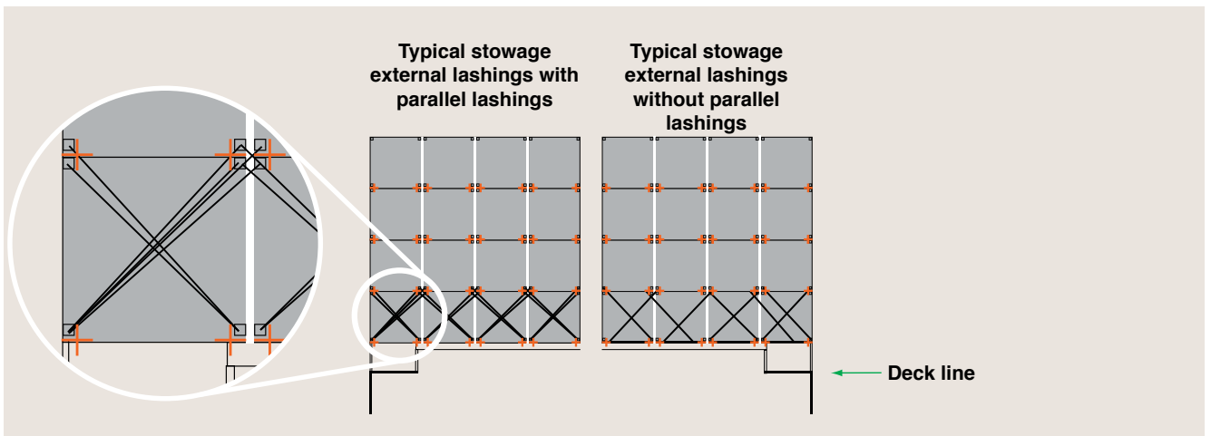
^ Containers secured by twistlocks and lashing rods, 'External lashing' arrangement
