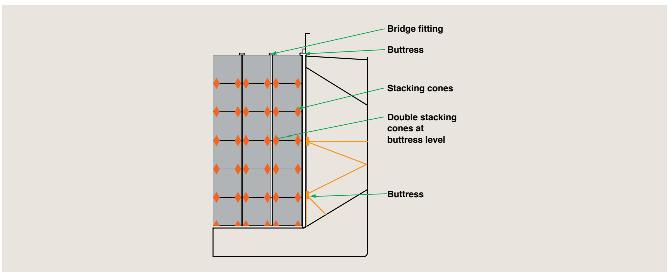
^ Typical bulk carrier stowage arrangement with buttresses, using single/double stacking cones and bridge fittings
