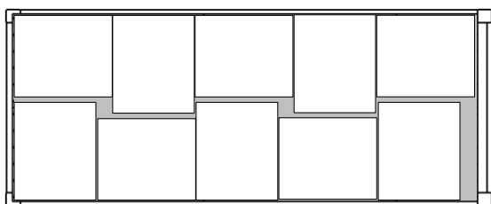
Figure 7.29 Packing 1,000 x 1,200 mm unit loads into a 20-foot container
